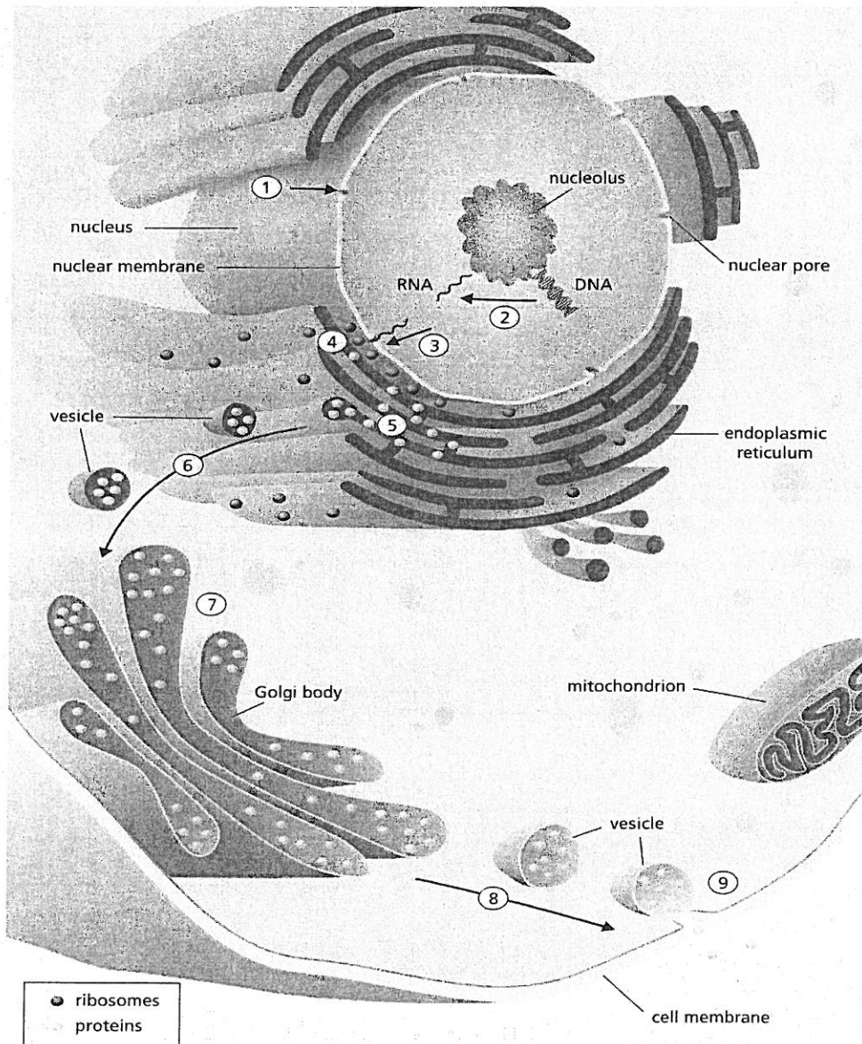
Figure 4.11 The production of a protein in an animal cell
